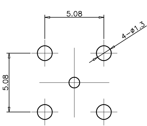
Mounting Detail
